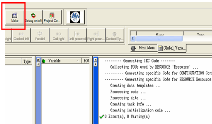
Fig. 5 Editing Screen
